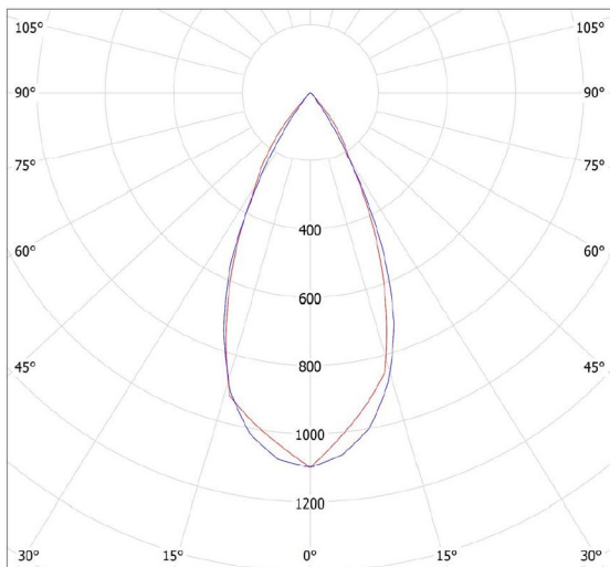
Light distribution (basis for the light distribution is 2500 lm / 4000 K)
