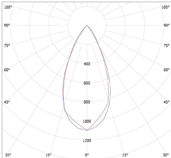
Light distribution (basis for the light distribution is 2500 lm / 4000 K)
